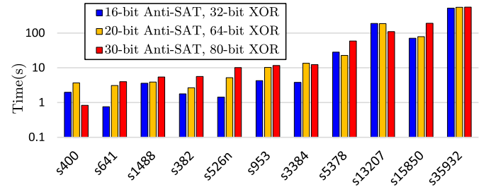
Fig. 4. Running time for decrypting unrolled ISCAS sequential benchmarks.
